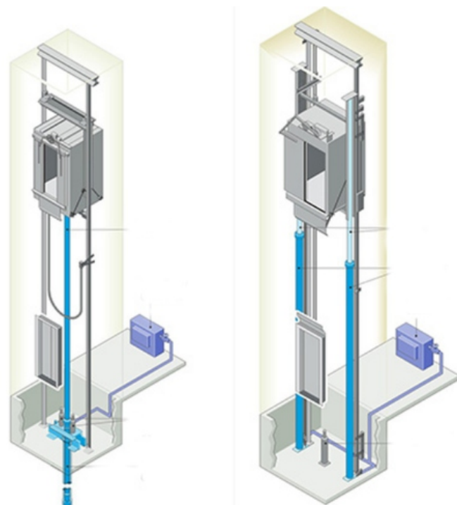
Hydraulic Elevator
